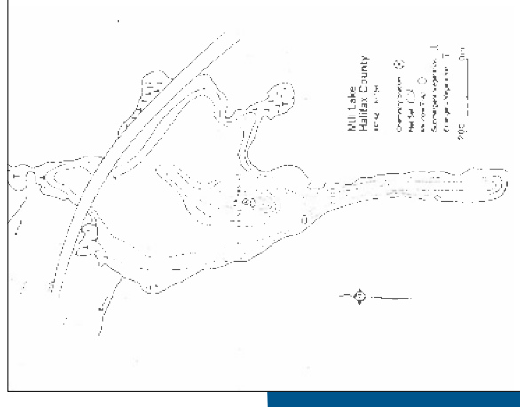
Bathymetry Map of Mill Lake
