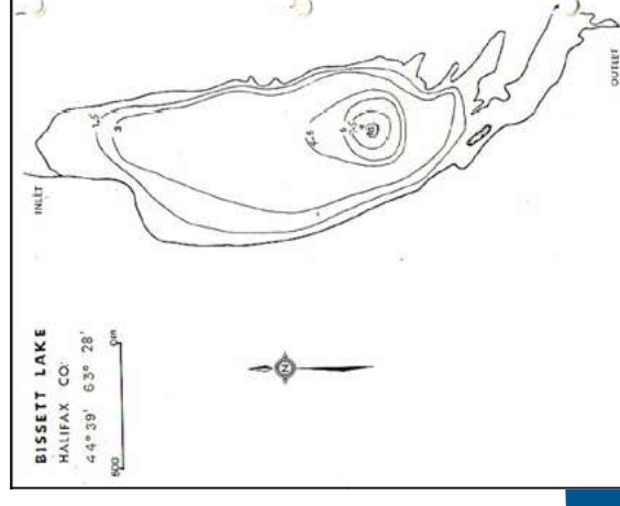
Bathymetry Map of Bissett Lake
