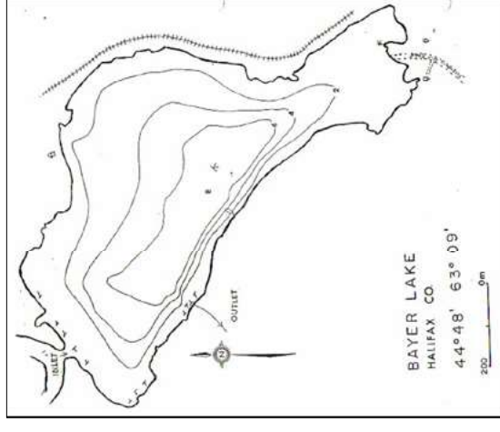
Bathymetry Map of Bayers Lake
