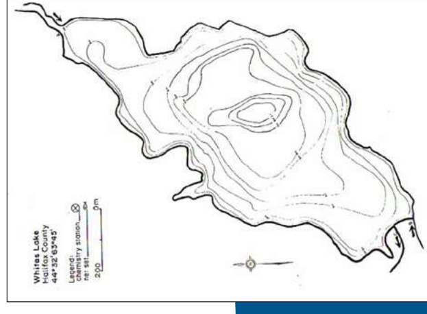
Bathymetry Map of Whites Lake
