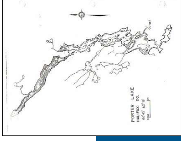
Bathymetry Map of Porters Lake
