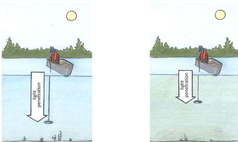
Figure 3. Example of different Secchi depth measurements due to differences in light penetration - Illustration provided courtesy of Atlantic DataStream ( https://datastream.org/en-ca/ )
