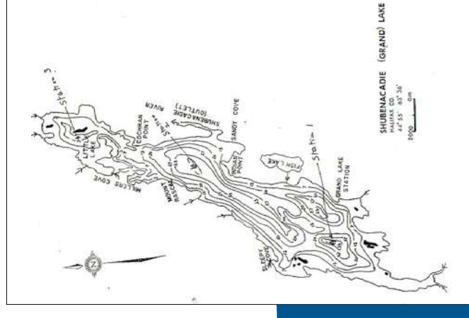
Bathymetry Map of Shubenacadie
