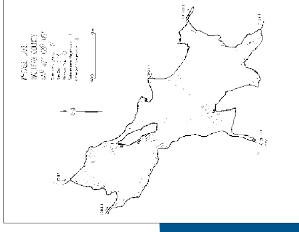
Bathymetry Map of McCabe Lake
