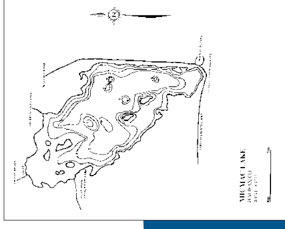
Bathymetry Map of Lake Micmac
