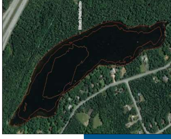
Bathymetry Map of Black Point Lake
