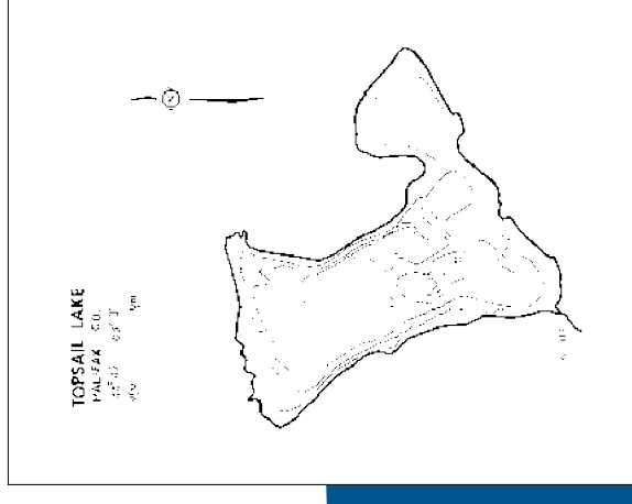
Bathymetry Map of Topsail Lake
