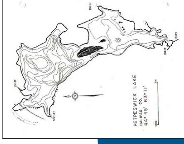
Bathymetry Map of Petpeswick Lake
