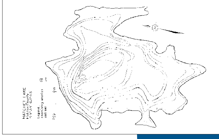
Bathymetry Map of Hatchet Lake
