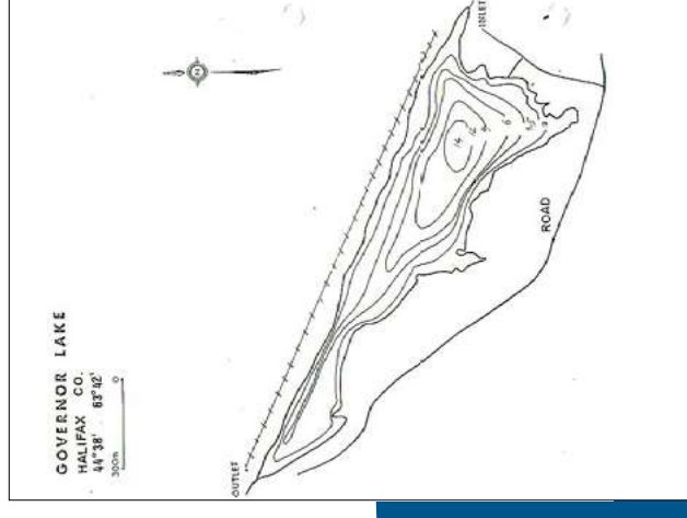
Bathymetry Map of Governor Lake
