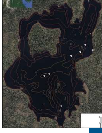
Bathymetry Map of Ragged Lake
