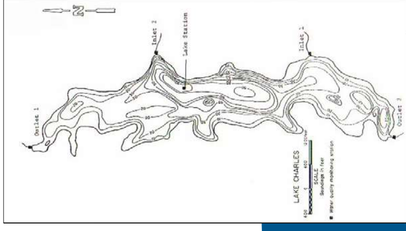
Bathymetry Map of Lake Charles
