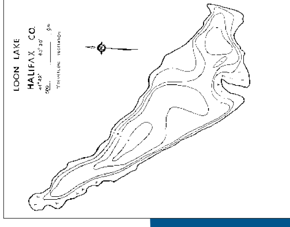
Bathymetry Map of Loon Lake
