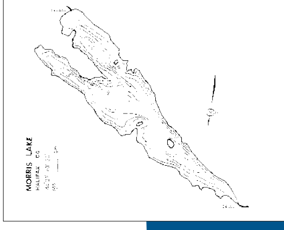
Bathymetry Map of Morris Lake
