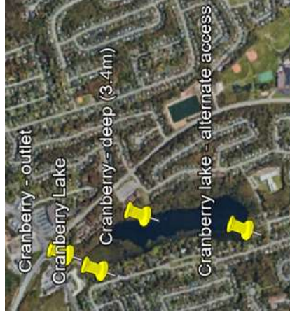
Satellite Imagery Map of Cranberry Lake w/ Sampling Locations
