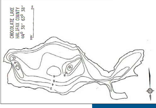
Bathymetry Map of Chocolate Lake
