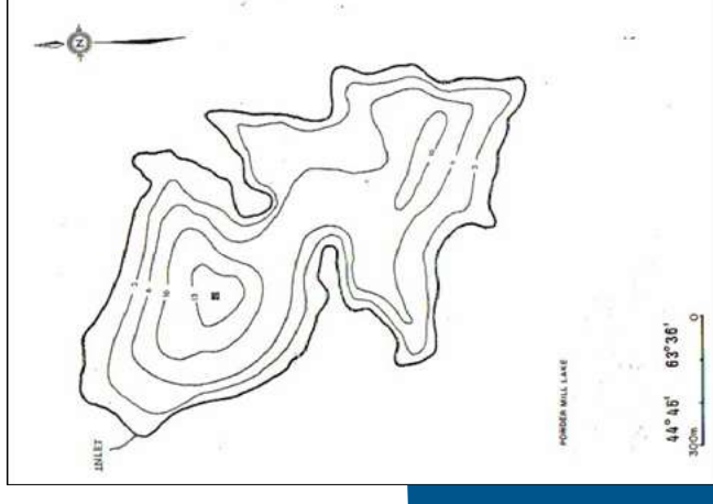
Bathymetry Map of Powder Mill Lake
