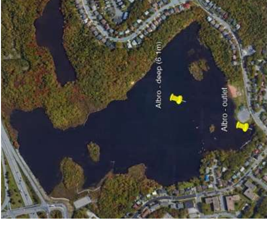
Satellite Imagery Map of Albro Lake w/ Sampling Locations
