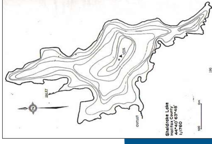
Bathymetry Map of Sheldrake Lake
