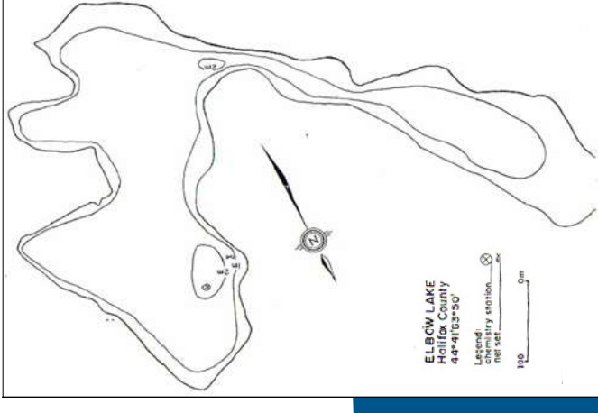
Bathymetry Map of Elbow Lake
