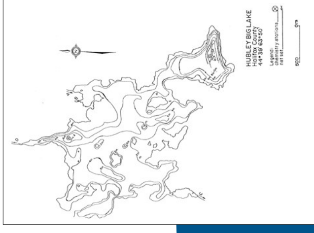
Bathymetry Map of Hubley Big Lake
