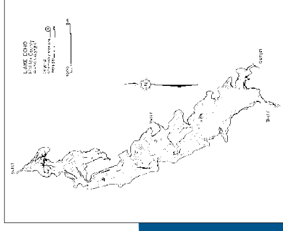
Bathymetry Map of Lake Echo
